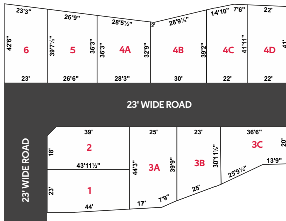
LAYOUT PLAN
